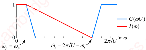
(e) Equivalent filter
